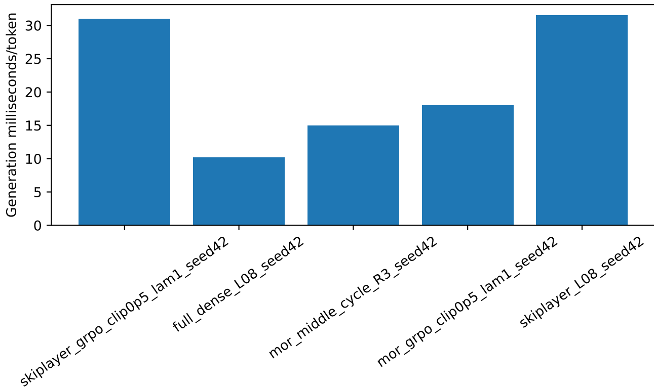
Generation milliseconds/token
