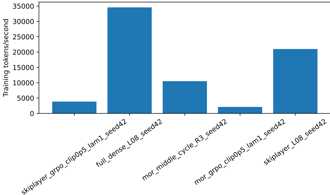
Training tokens/second
