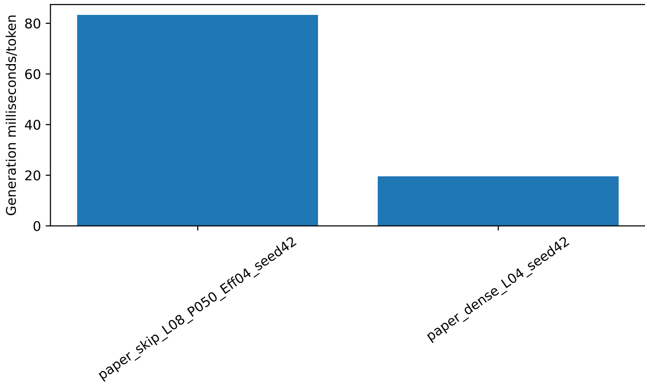
Generation milliseconds/token
