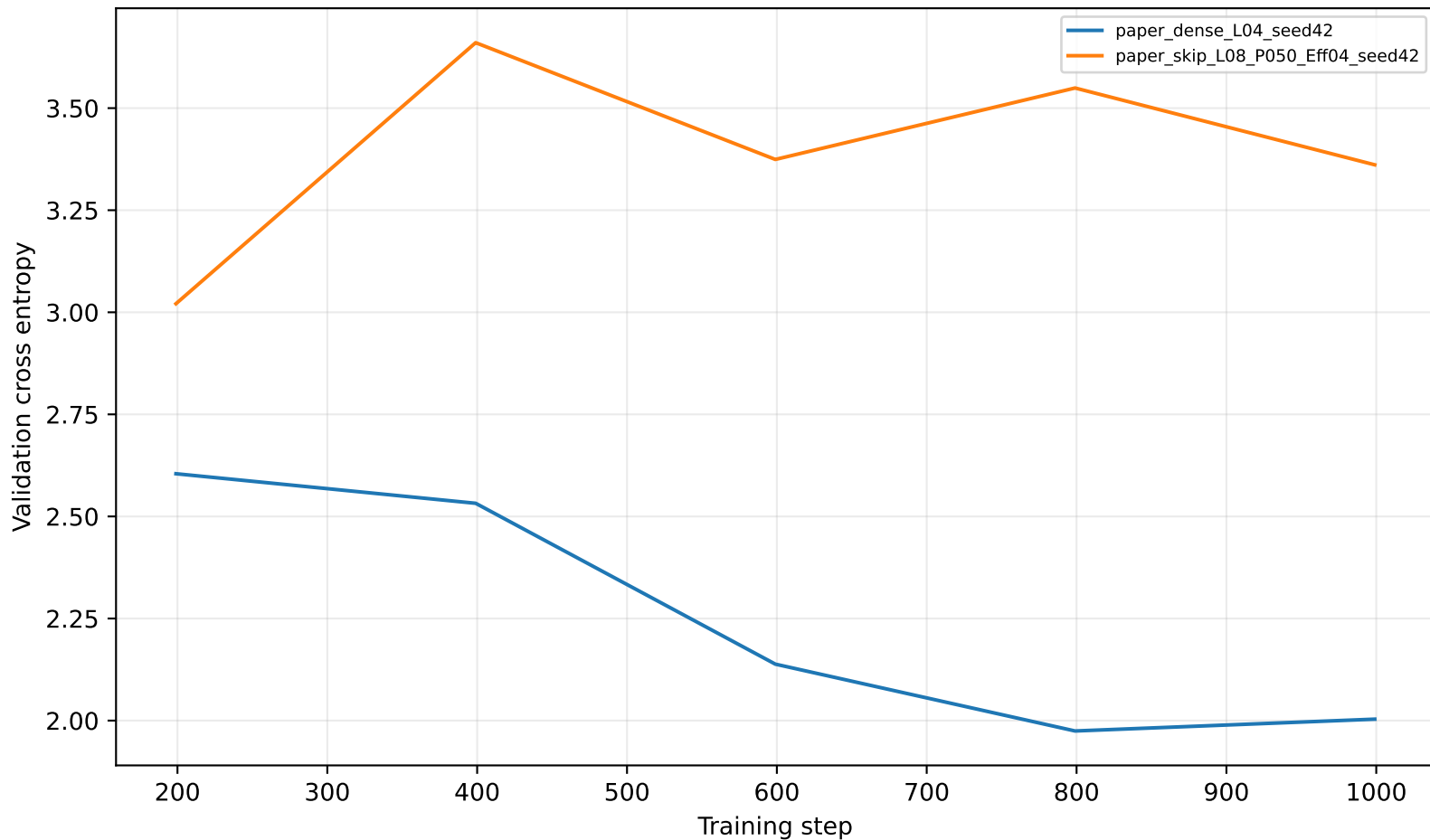
Validation cross entropy across experiments
