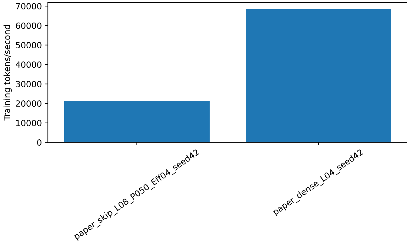
Training tokens/second
