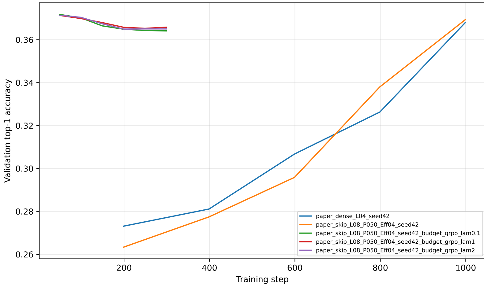
Validation top-1 accuracy across experiments
