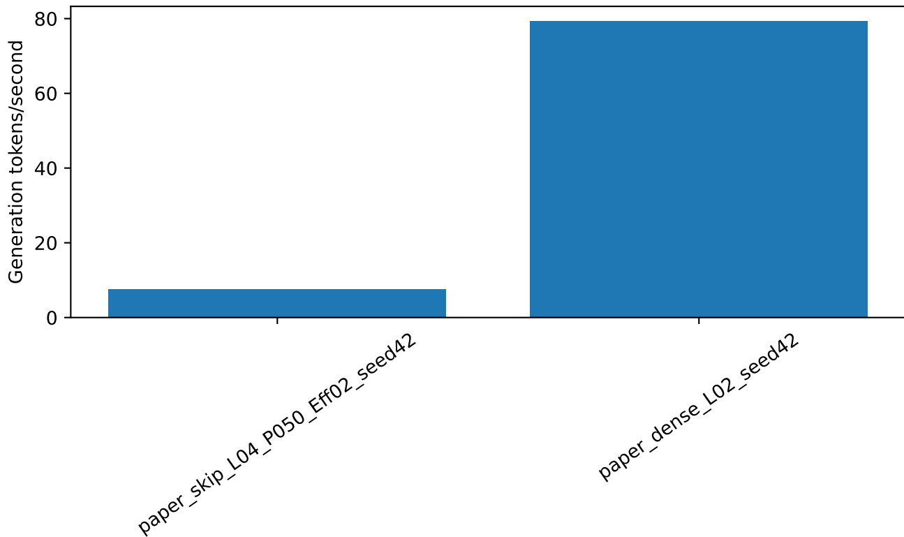
Generation tokens/second
