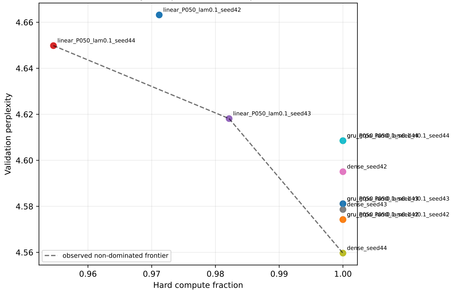
Quality-compute Pareto comparison
