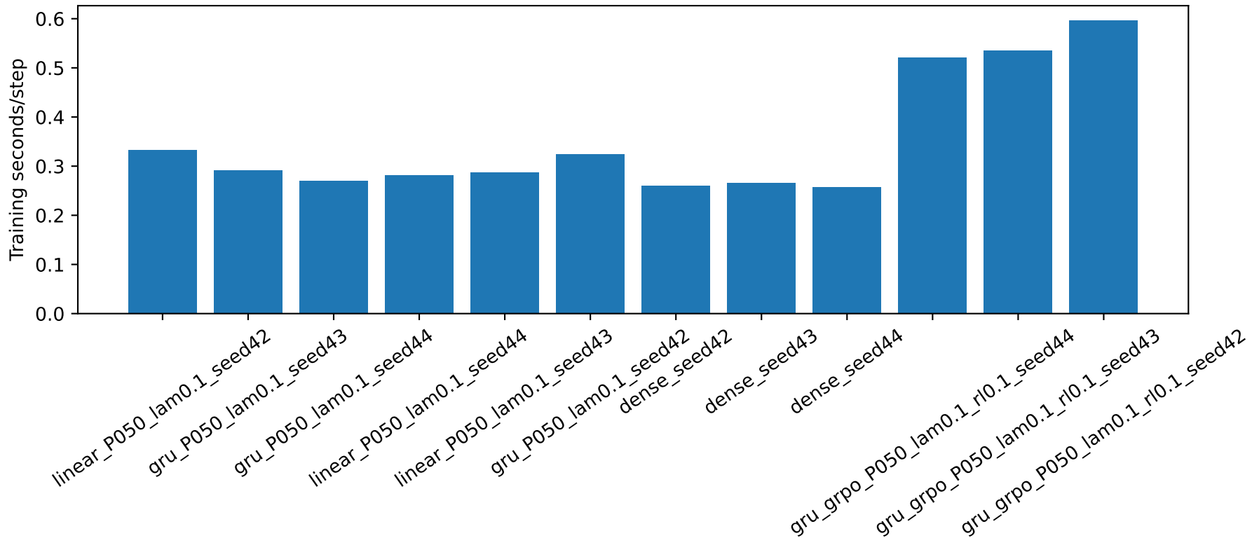
Training seconds/step
