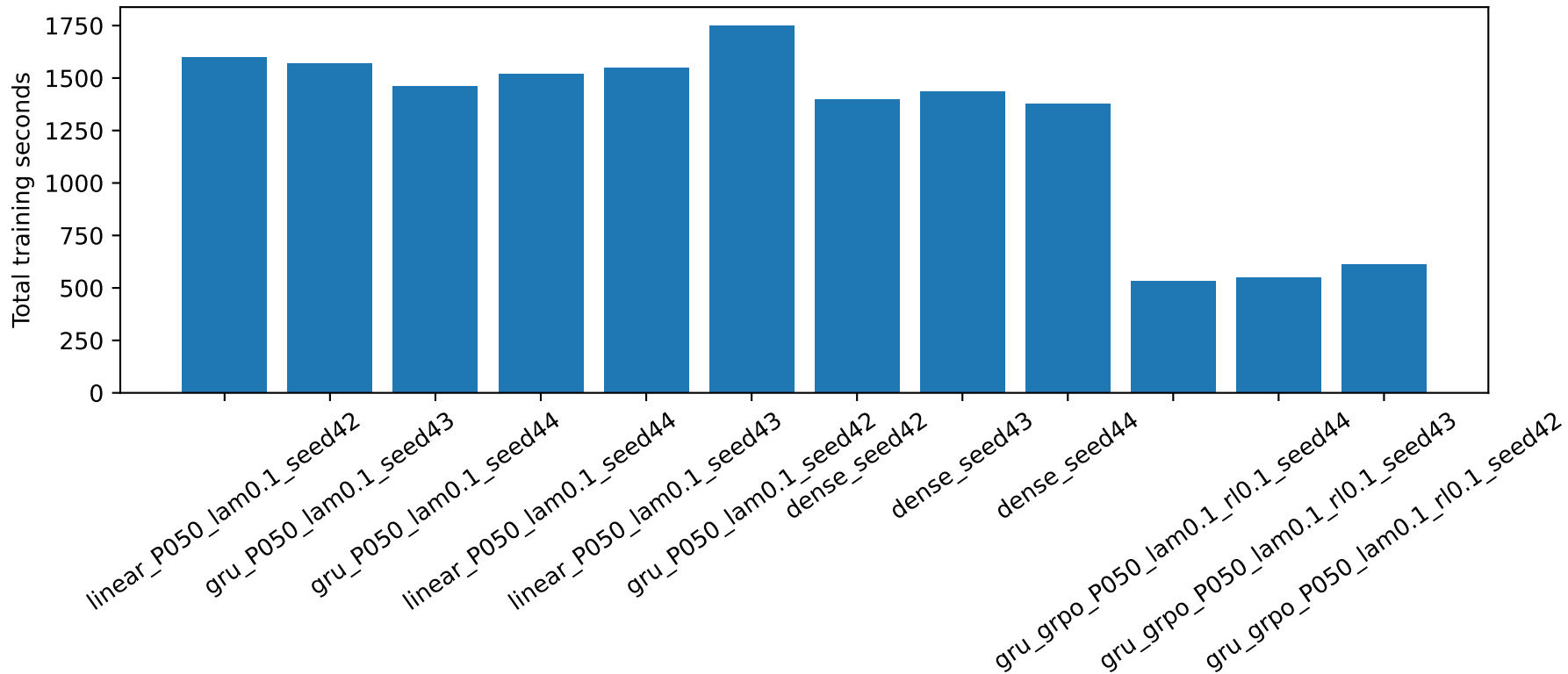
Total training seconds
