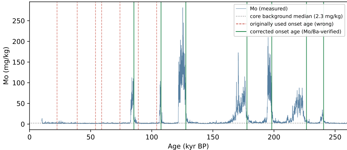
Core 64PE406E1: molybdenum record with original vs. corrected sapropel ages
