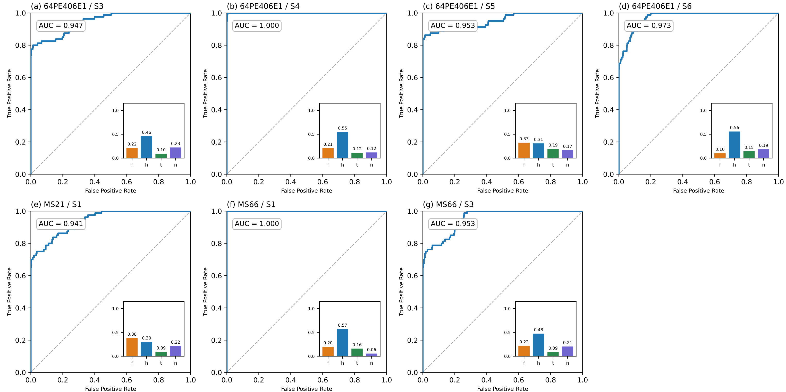
Trustworthy-ensemble ROC and favoured bifurcation type, by sapropel (Bury et al. 2021, Fig. 2 style)
