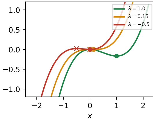
Transcritical: stability exchanges
