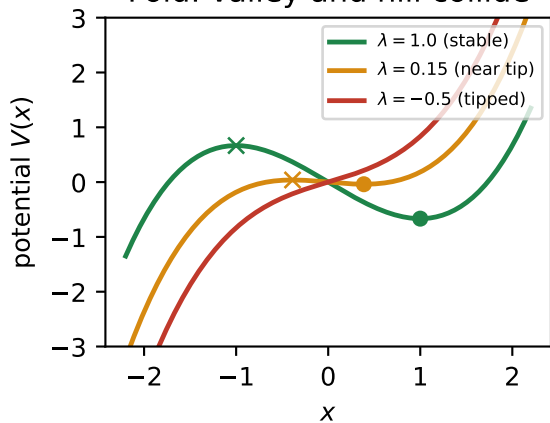
Fold: valley and hill collide
