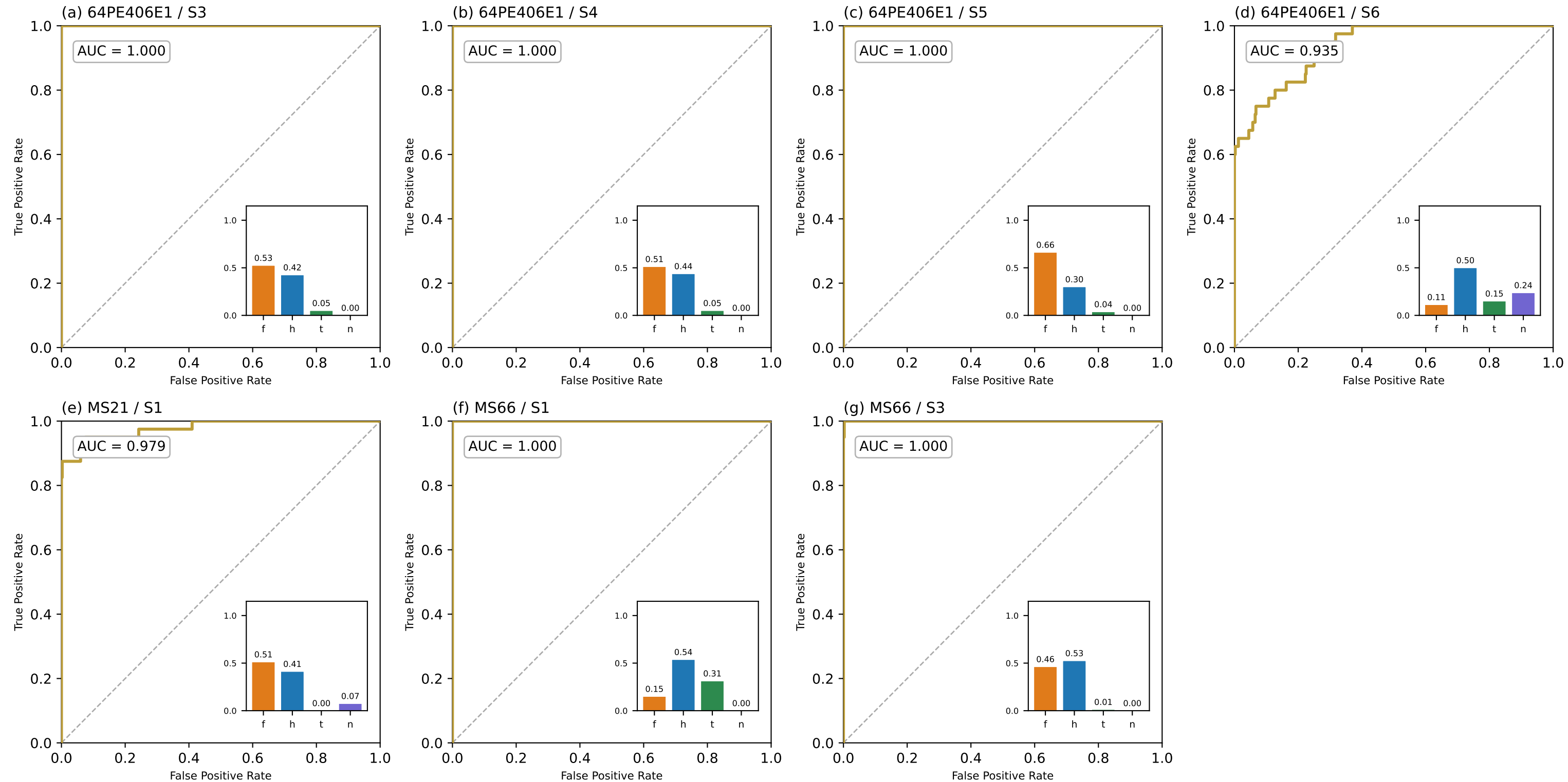
resnet — Mo — ROC and favoured bifurcation type, by sapropel
