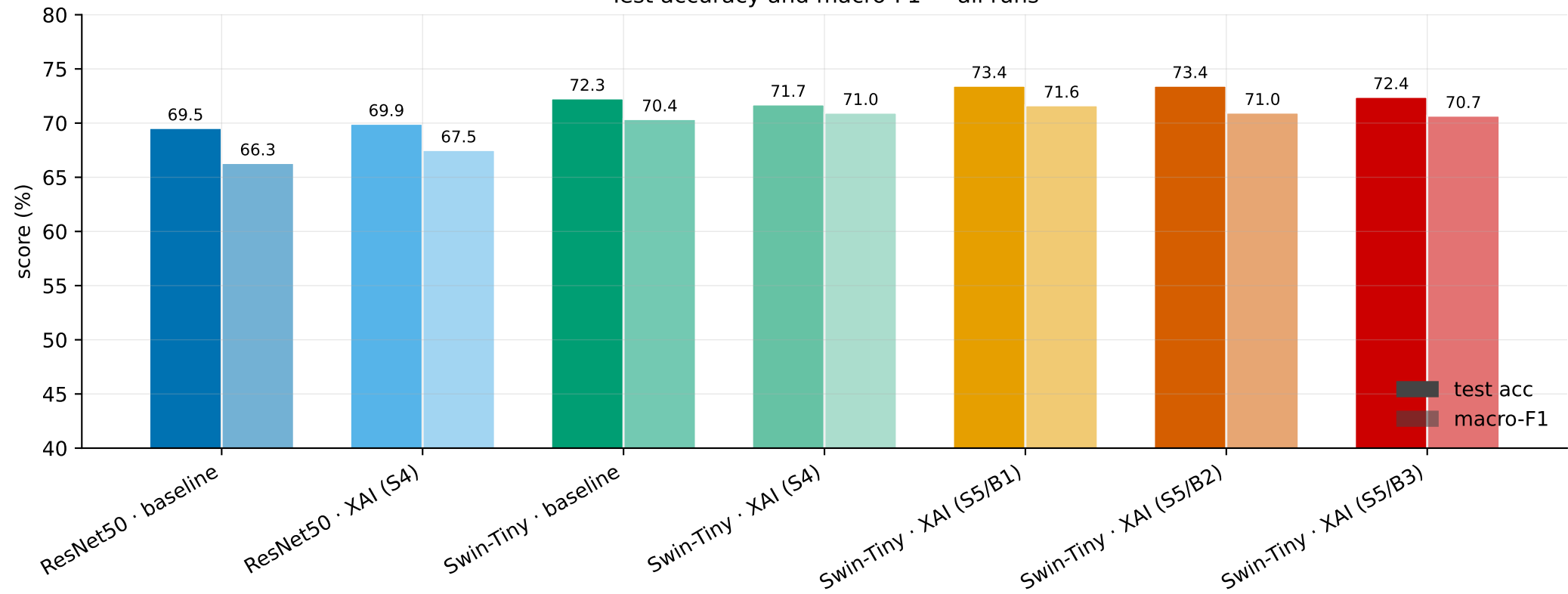
Test accuracy and macro-F1 — all runs
