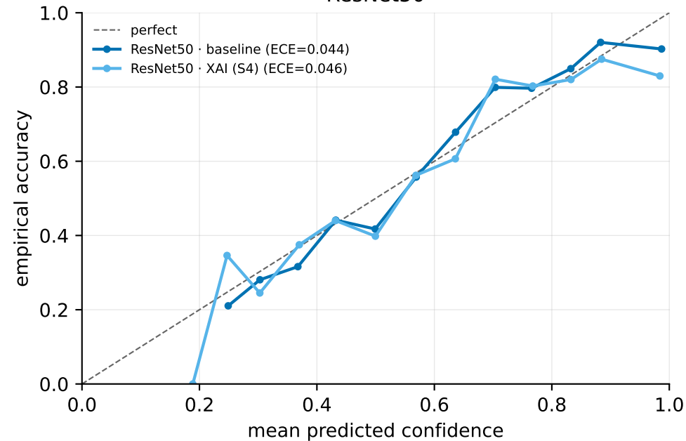
ResNet50
