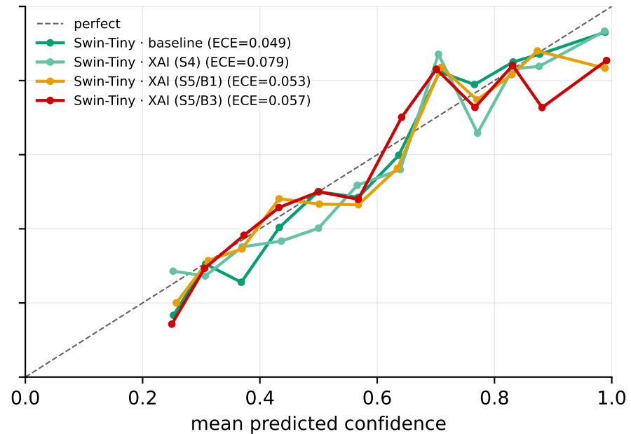
Swin-Tiny
