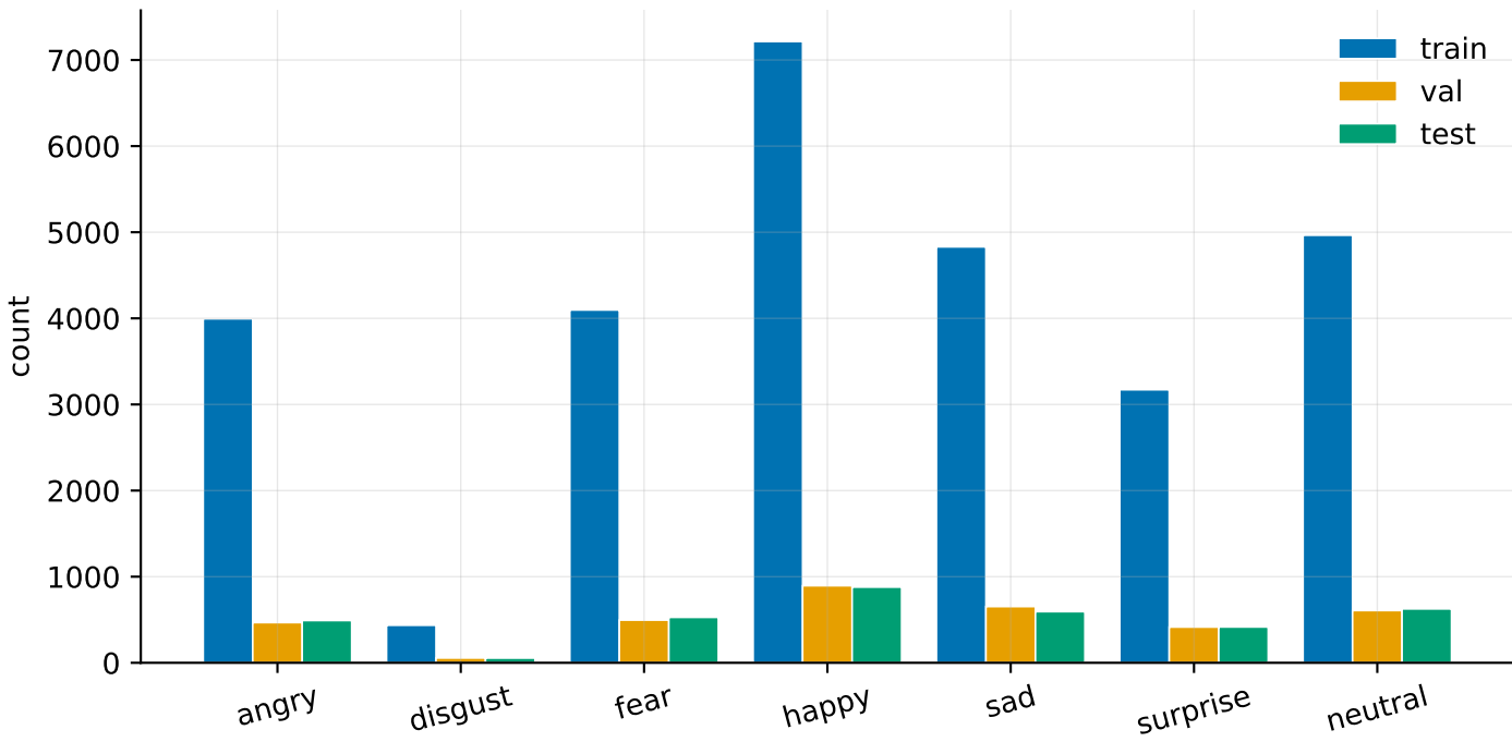
FER2013 class distribution by split
