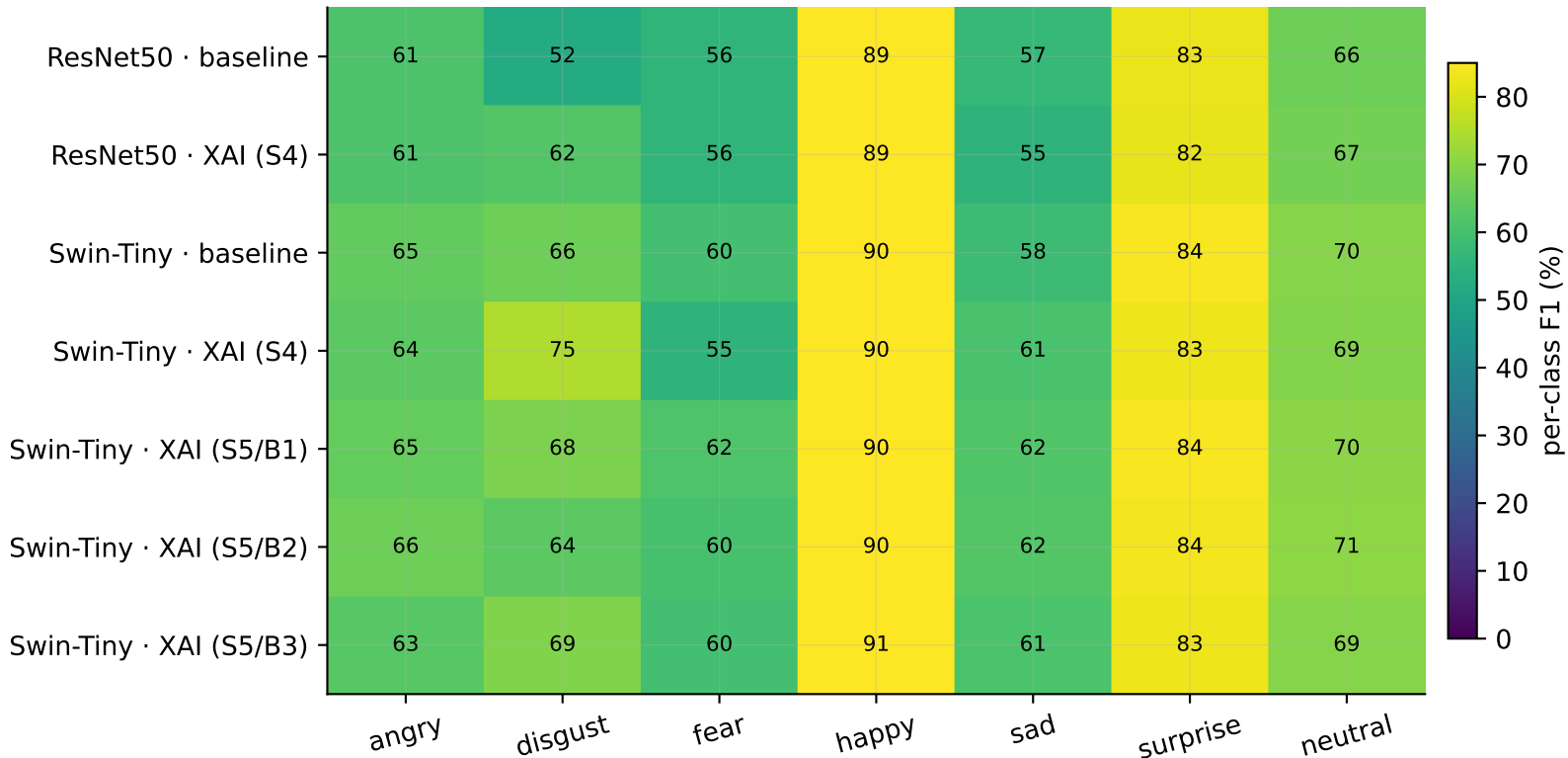
Per-class F1 score across runs
