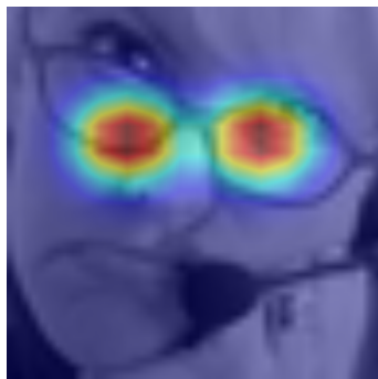
anatomical mask
