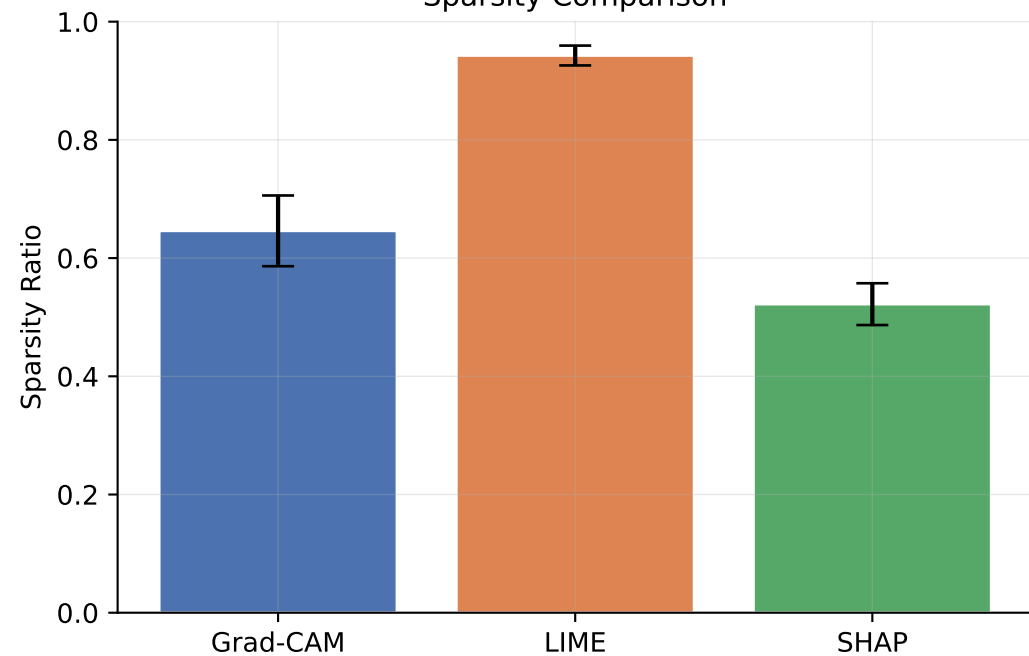
Sparsity Distribution
