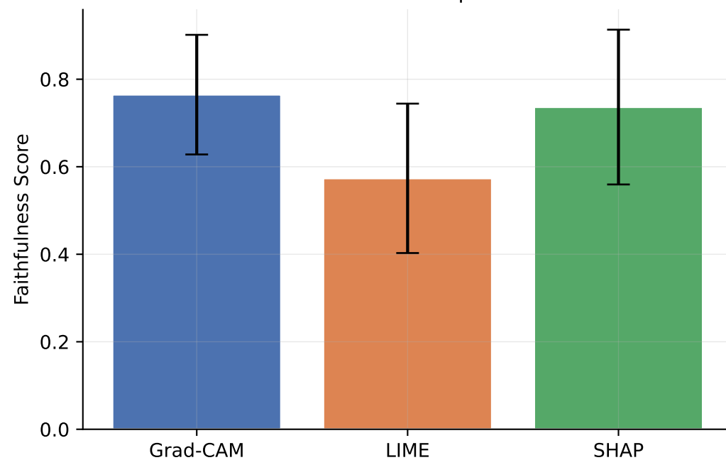
Faithfulness Distribution
