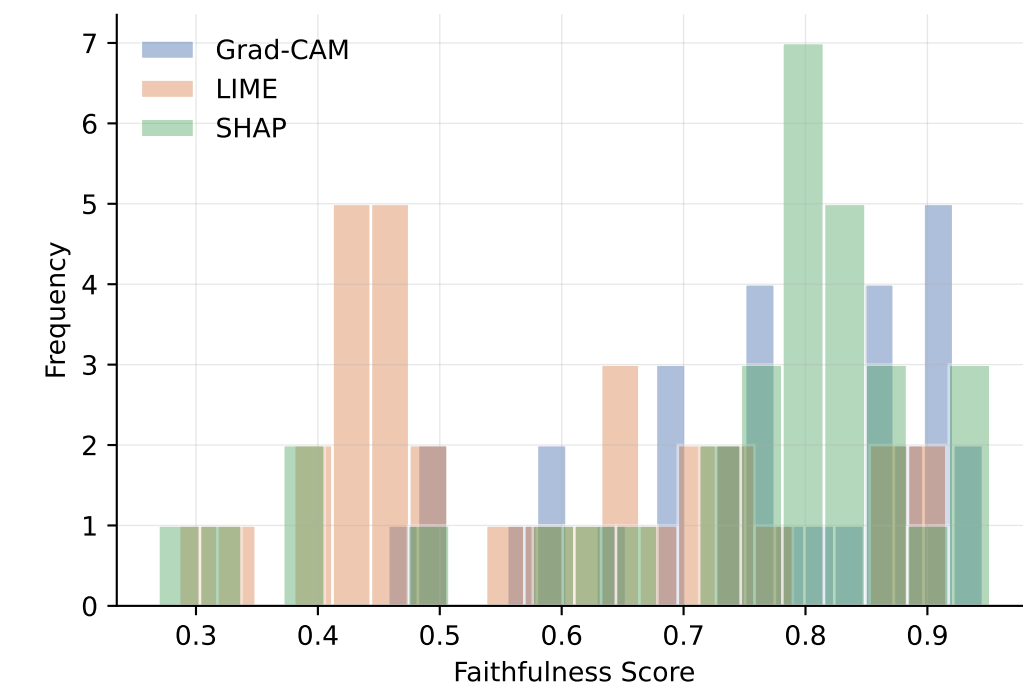
Faithfulness Distribution
