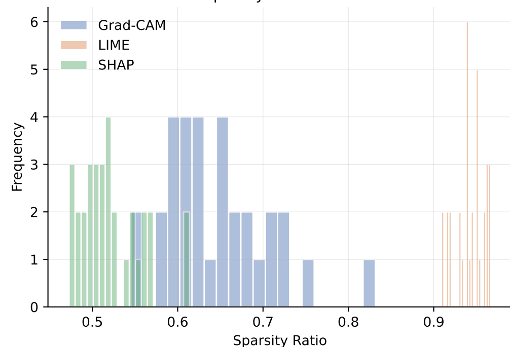
Sparsity Distribution
