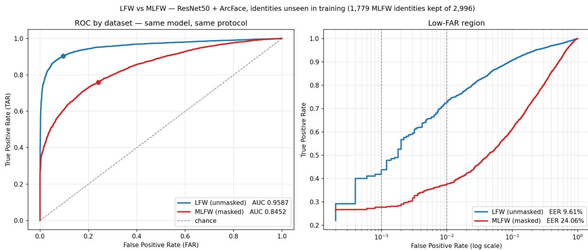
Figure 6 - ROC per dataset under one model and one protocol. Left: linear axes. Right: the low-FAR region, where the mask penalty is largest.
