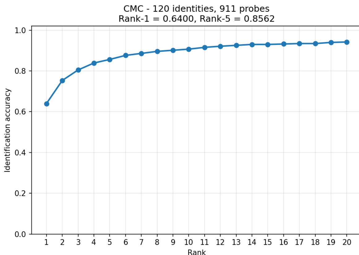
Figure 5 - CMC curve: probability the correct identity is within the top-k gallery matches.
