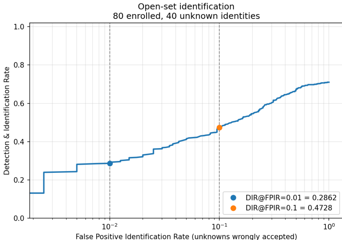
Figure 6 - Detection & identification rate against the rate at which unknown people are wrongly accepted.
