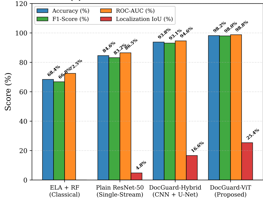
(a) Performance Across 4 Models
