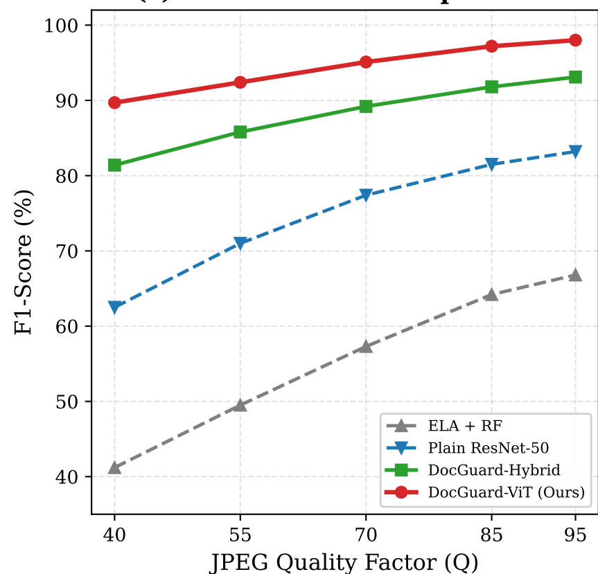
(c) Robustness to Compression
