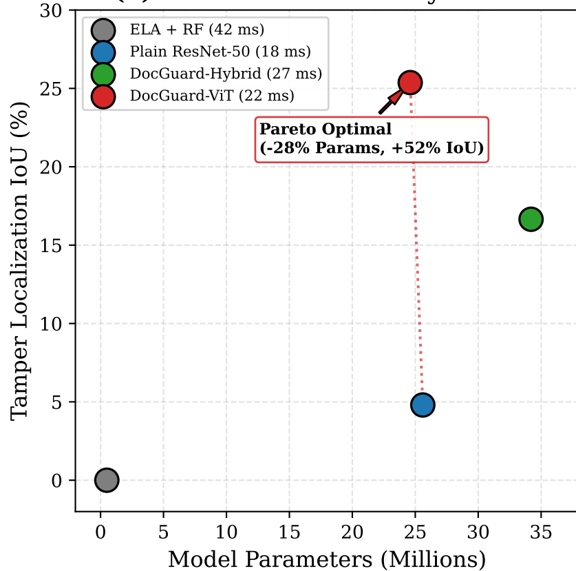
(b) Parameter Efficiency vs. IoU
