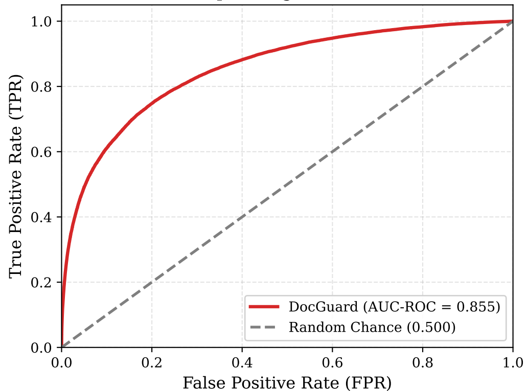
(b) Receiver Operating Characteristic (ROC)
