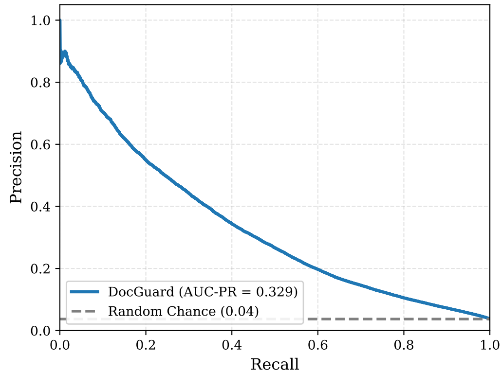
(a) Pixel-Level Precision-Recall (PR)
