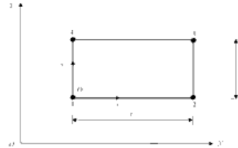
Fig. 5.28 A four-noded rectangular element.
