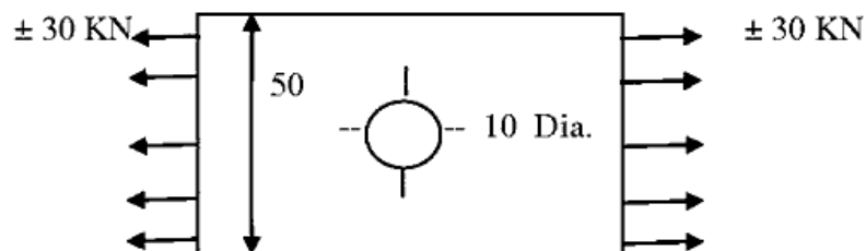
Figure 2. ( All dimensions are in mm )
