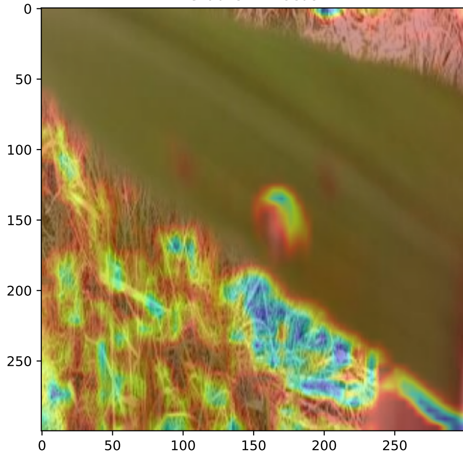
Grad-CAM Focus
