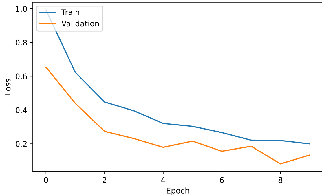
CNN - Loss
