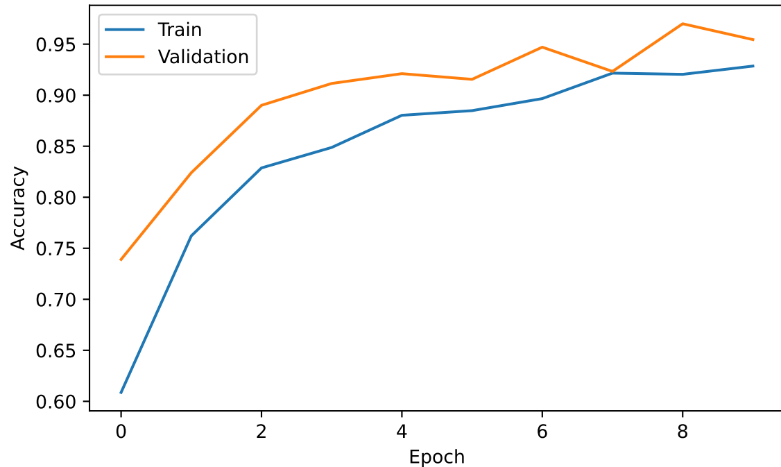
CNN - Accuracy
