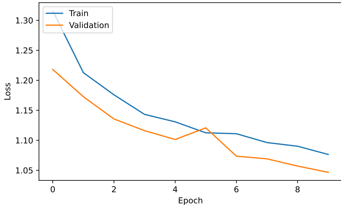
ResNet50 - Loss
