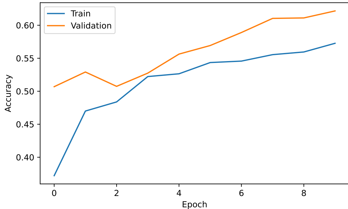
ResNet50 - Accuracy
