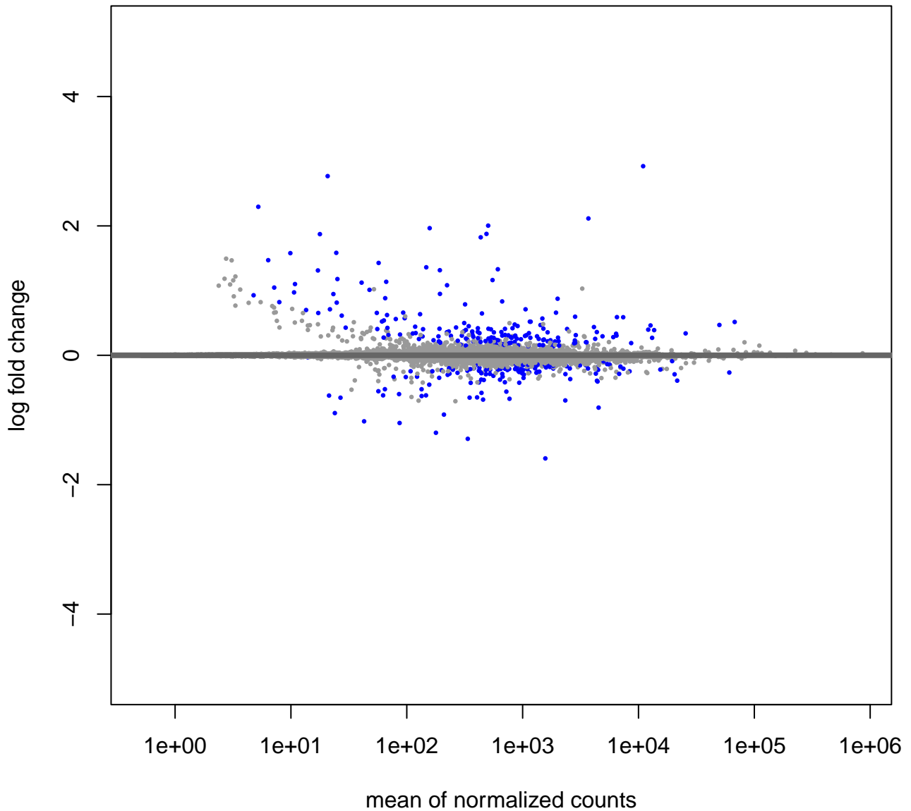
MA Plot (Shrunken LFC)
