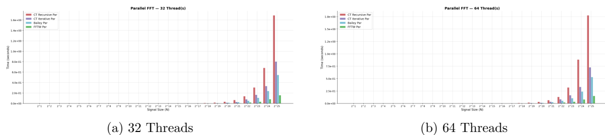
Figure 4: Parallel FFT Execution Times (32 and 64 Threads)
