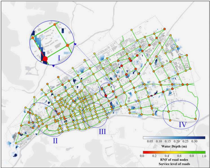
Fig 6. An inundation instance and concurrent RNF in Ling-Xi.
