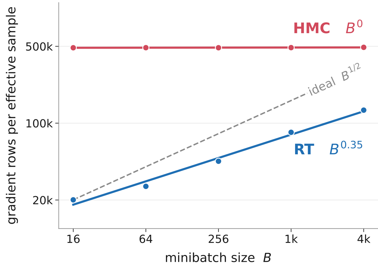
(b) real minibatches
