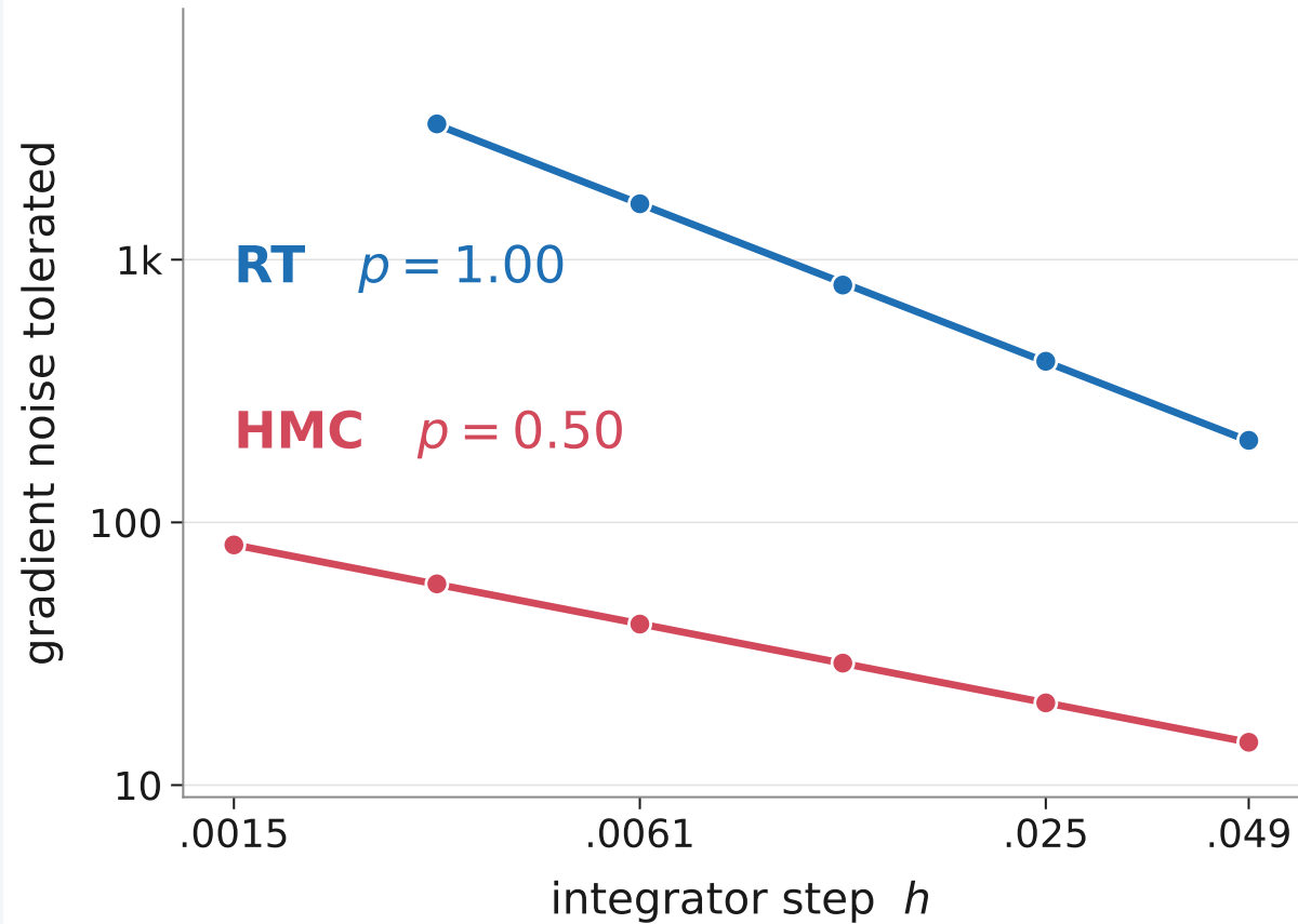
(a) controlled Gaussian noise
