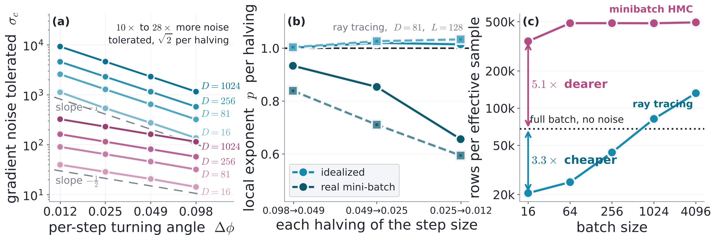
(a) isotropic jitter, exact Gaussian target. (b) matched-condition arms; solid synthetic, dashed superconductor. (c) UCI superconductivity.
