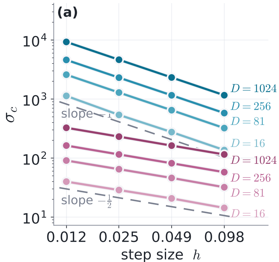
Idealized isotropic gradient noise
