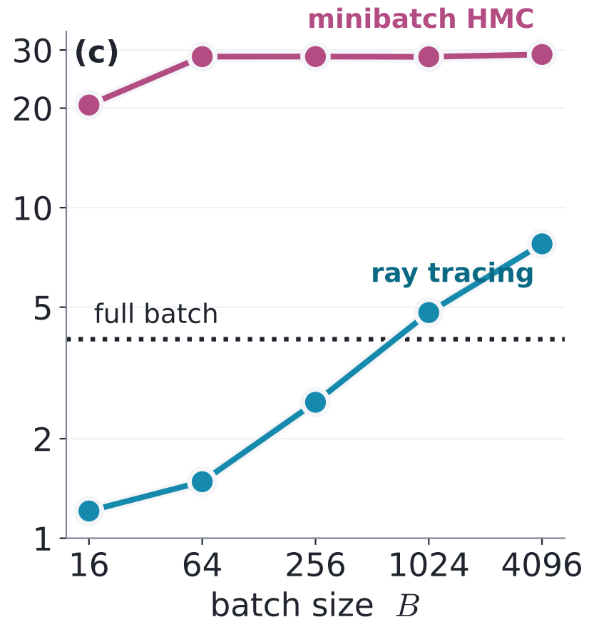
UCI Superconductivity dataset
