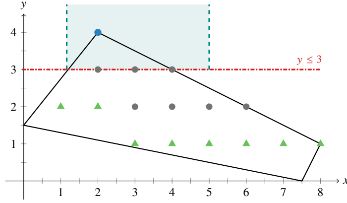
Figure 12.4 An illustration of an improving solution intersection cut for the bilevel problem in Example 12.21. Starting with the optimal solution (2, 4) to the single-level relaxation and the improving solution of the follower \hat{y} = 3 for x^* = 2 found by solving Problem (12.9), we derive the intersection cut y \leq 3 from the improving solution bilevel-free set \mathcal{T}^+(\hat{y}) = \{(x, y) : 29/25 \leq x \leq 5, y \geq 3\} . The shaded area corresponds to \mathcal{T}^+(\hat{y}) . The dash-dotted line represents the intersection cut.
