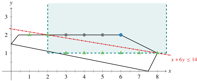
Figure 12.2 An illustration of an improving solution intersection cut for the bilevel problem in Example 12.8. Starting with the LP cone of the optimal solution (6, 2) to the single-level relaxation and intersecting it with \mathcal{T}^+(1) , we derive the intersection cut x + 6y \leq 14 . The shaded area corresponds to the bilevel-free set \mathcal{T}^+(1) . The dash-dotted line represents the intersection cut.
