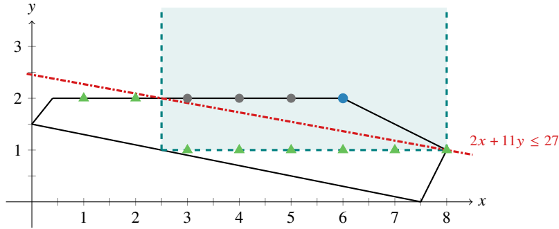
Figure 12.1 An illustration of an improving solution intersection cut for the bilevel problem in Example 12.8. Starting with the LP cone of the optimal solution (6, 2) to the single-level relaxation and intersecting it with \mathcal{T}(1) , we derive the intersection cut 2x + 11y \leq 27 . The shaded area corresponds to the bilevel-free set \mathcal{T}(1) . Note that the boundary y = 1 is excluded from \mathcal{T}(1) because the strict inequality y > 1 defines an open set. The dash-dotted line represents the intersection cut.
