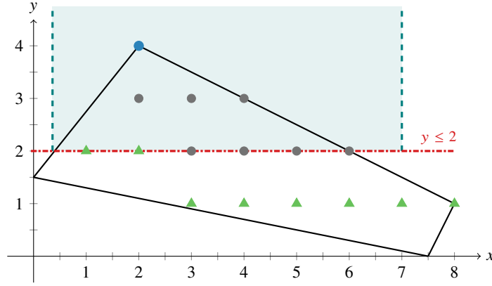
Figure 12.3 An illustration of an improving solution intersection cut for the bilevel problem in Example 12.21. Starting with the optimal solution (2, 4) to the single-level relaxation and the optimal follower's response \hat{y} = 2 for x^* = 2 , we derive the intersection cut y \leq 2 from the improving solution bilevel-free set \mathcal{T}^+(\hat{y}) = \{(x, y) : 9/25 \leq x \leq 7, y \geq 2\} . The shaded area corresponds to the bilevel-free set \mathcal{T}^+(\hat{y}) . The dash-dotted line represents the intersection cut.
