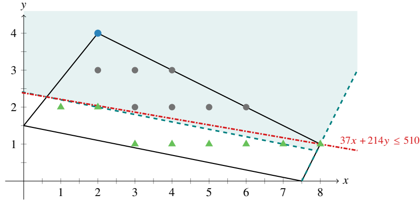
Figure 12.5 An illustration of an improving direction intersection cut for the bilevel problem in Example 12.22. Starting with the optimal solution (2, 4) to the single-level relaxation, we derive the intersection cut 37x + 214y \leq 510 from the improving direction bilevel-free set X^+(\Delta\hat{y}) = \{(x, y) : 2x - y \leq 15, -2x - 10y \leq -24\} . Dashed lines are faces of the set X^+(\Delta\hat{y}) . The dash-dotted line represents the intersection cut.
