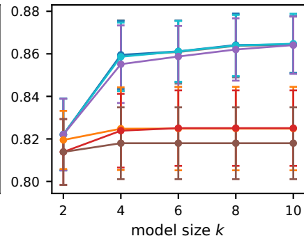
mammographic (n=581, p=11)
