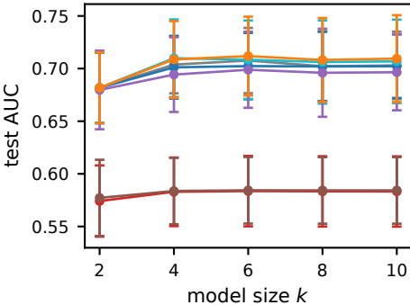
ilpd (n=408, p=11)
