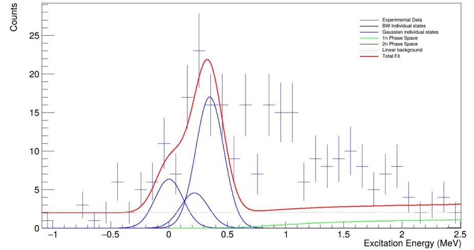
^{17}\text{C} Spectrum for 35-40° in c.m.
