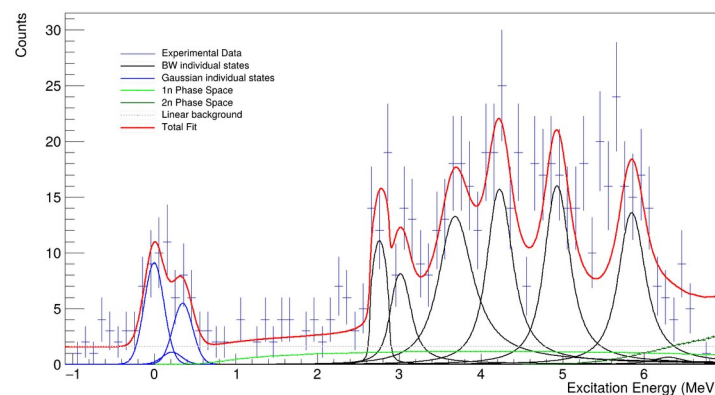
^{17}\text{C} Spectrum for 25-30° in c.m.
