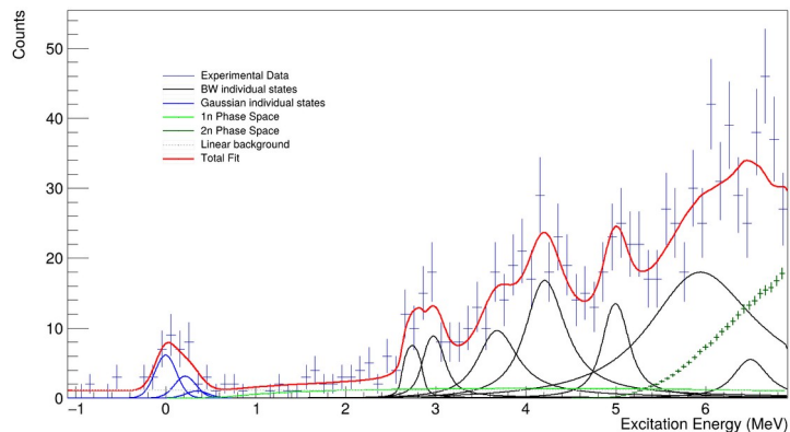
^{17}\text{C} Spectrum for 20-25° in c.m.
