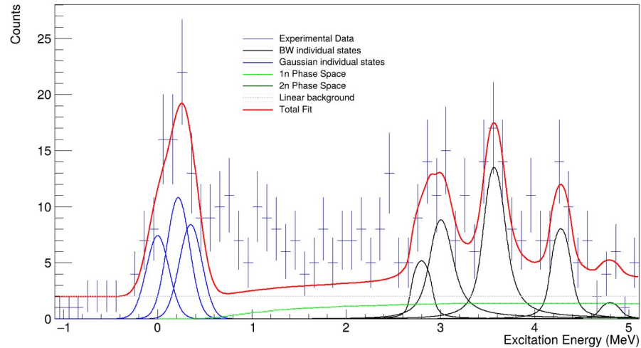
^{17}\text{C} Spectrum for 30-35° in c.m.
