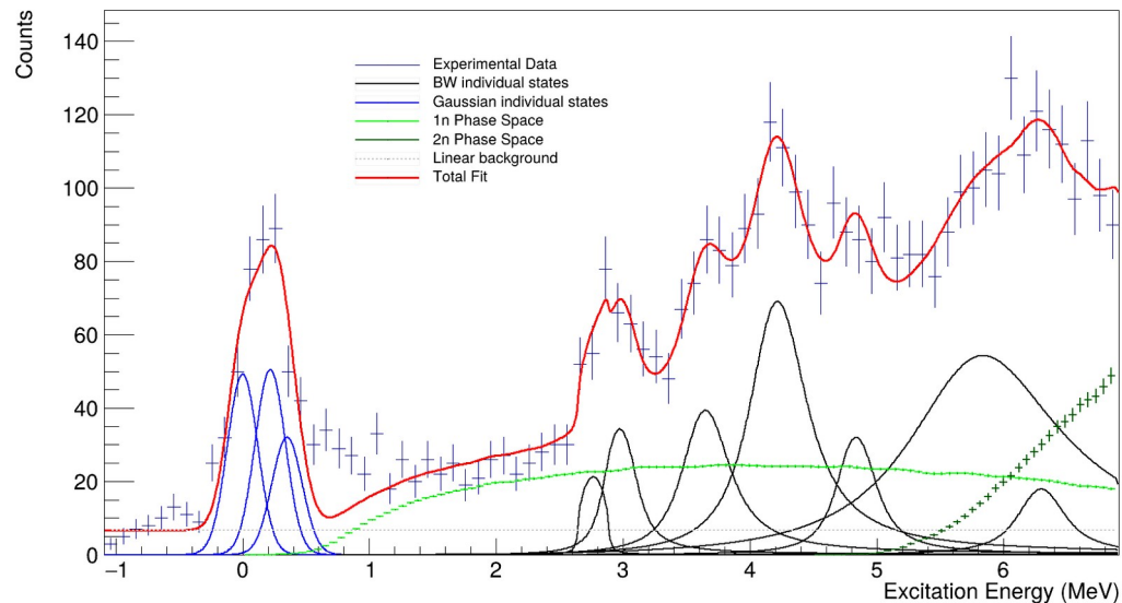
^{17}\text{C} Spectrum
