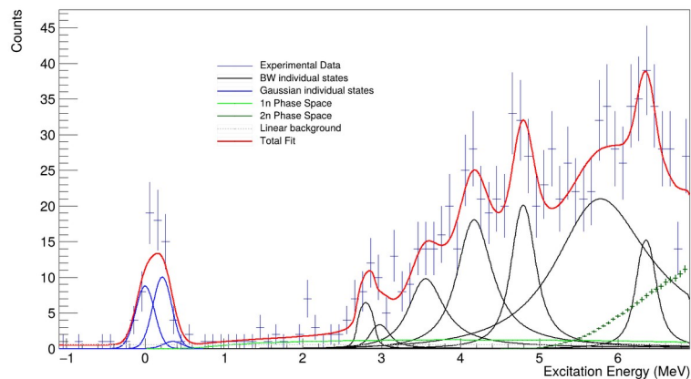
^{17}\text{C} Spectrum for 20-25° in c.m.
