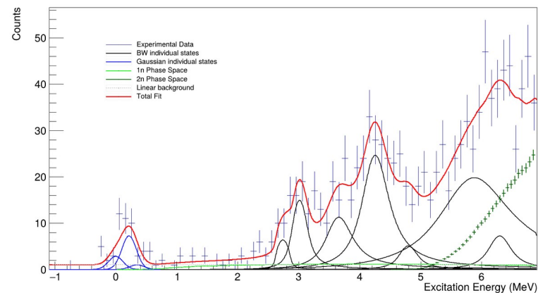
^{17}\text{C} Spectrum for 25-30° in c.m.
