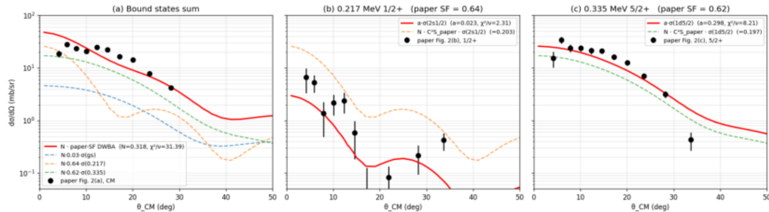
^{16}\text{C}(\text{d},\text{p})^{17}\text{C} — paper's CM angular distributions vs our FRESKO DWBA \times paper SFs global N = 0.318 (ADWA-vs-DWBA + energy difference: 17.2 vs 11.77 MeV/u)
