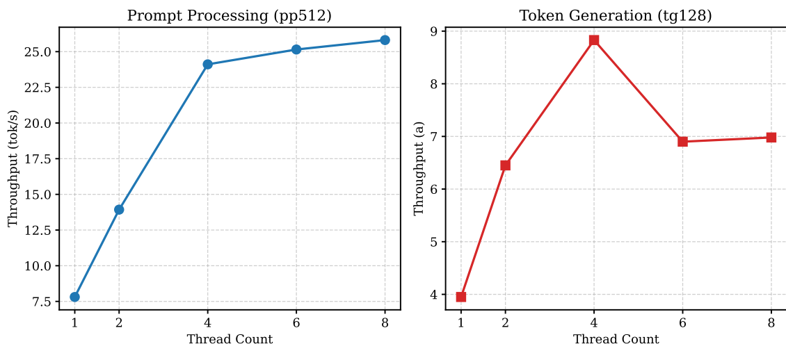
Figure 3.1: Ryzen 5600H: prefill saturates near the physical core count; generation retrogrades past 4 threads.
