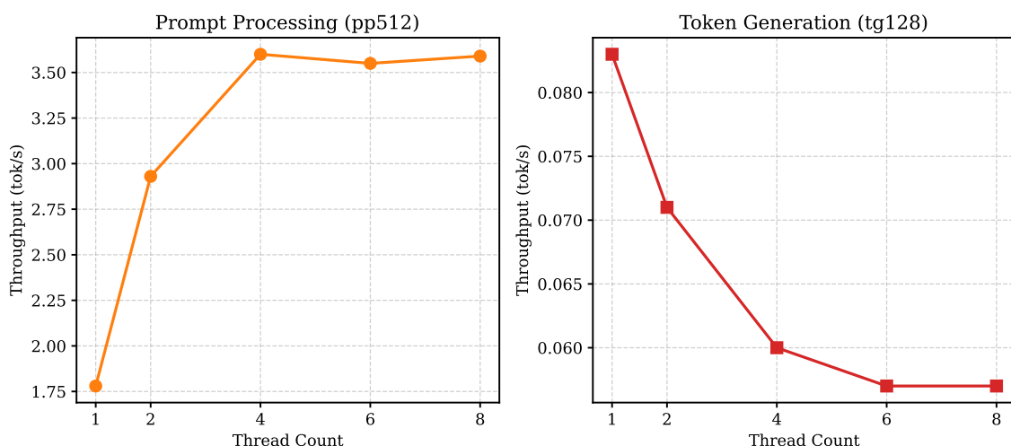
Figure 3.2: Pentium G5420: prefill saturates by 4 threads; generation retrogrades monotonically.
