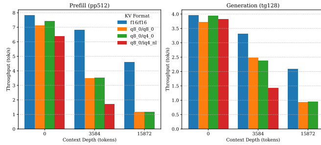
Figure 3.4: Ryzen 5600H, 1 thread: every quantized-KV configuration was slower than f16, worsening with context depth.
