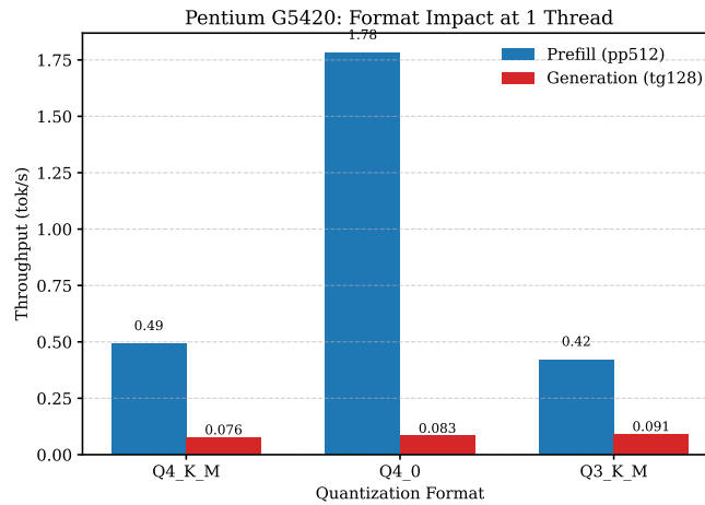
Figure 3.5: Pentium G5420, 1 thread: quantization format , not just bit-width, determines CPU throughput.
