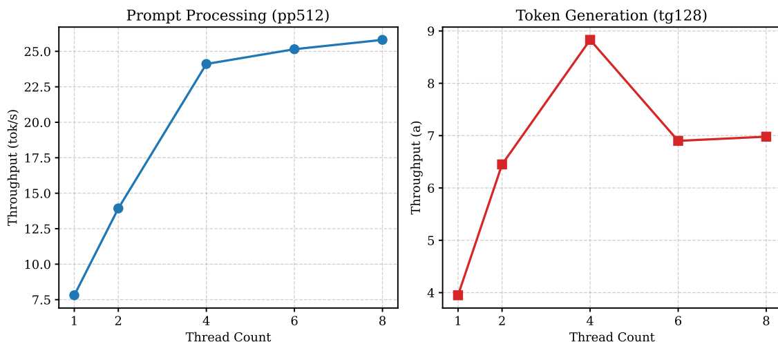
Figure 3.1: Ryzen 5600H: prefill saturates near the physical core count; generation retrogrades past 4 threads.
