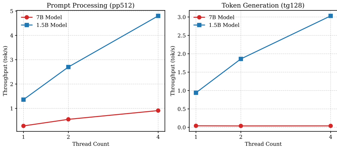
Figure 3.3: Jetson Nano: prefill scales for both models; generation only scales for the smaller one.
