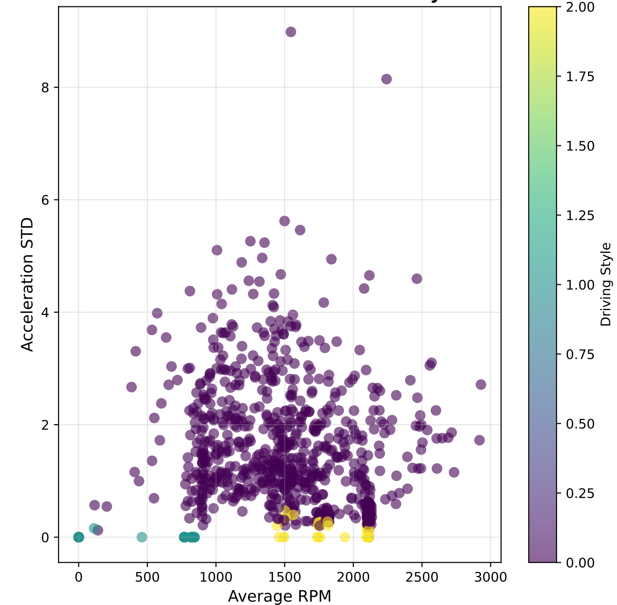
RPM vs Acceleration Variability
