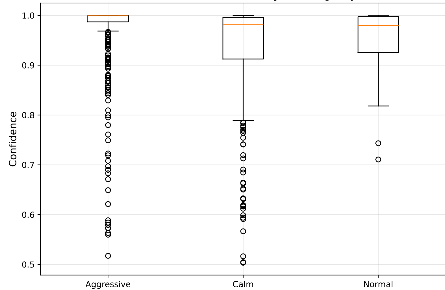
Prediction Confidence by Driving Style
