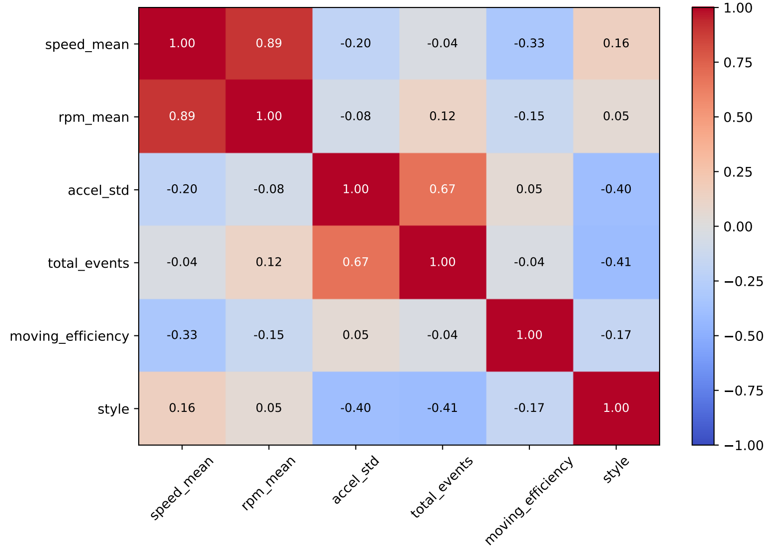
Feature Correlation Matrix
