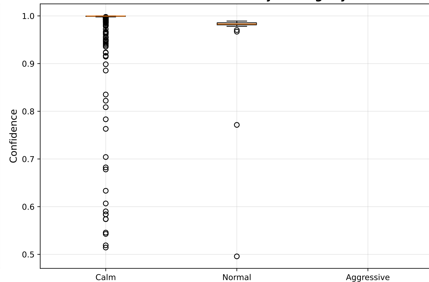
Prediction Confidence by Driving Style
