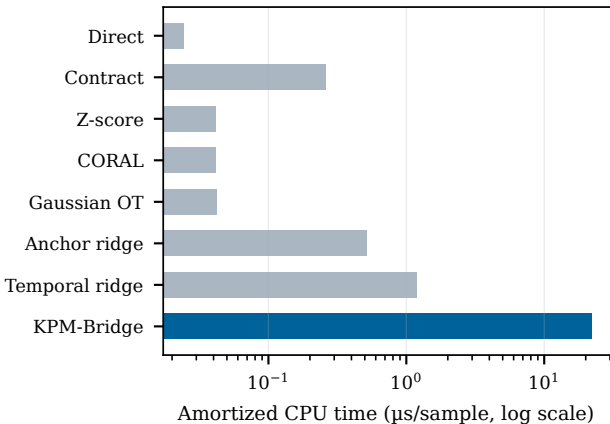
Batched reference implementation
