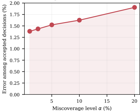
Risk paid for lower abstention
