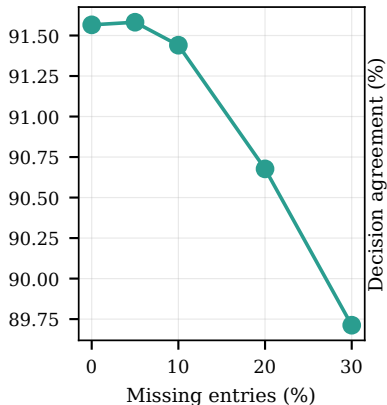
Missingness stress
