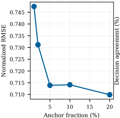
Paired-anchor budget
