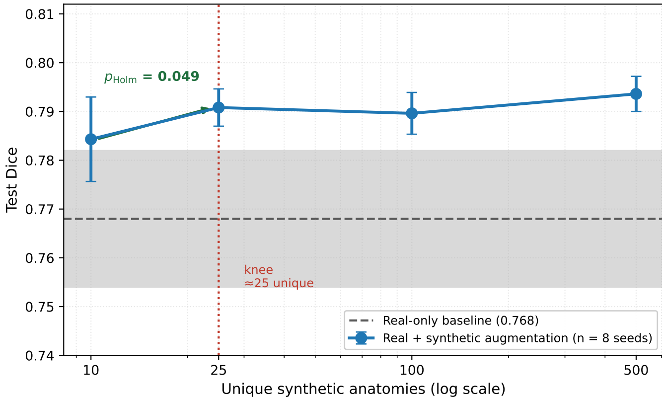
Diversity dose-response: 18 real + 500 synthetic (total count fixed; only the unique count varies)
