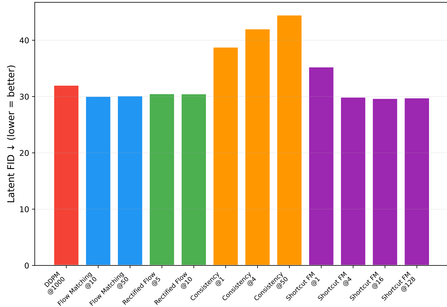
(b) Fréchet Distance in VQ-GAN Latent Space
