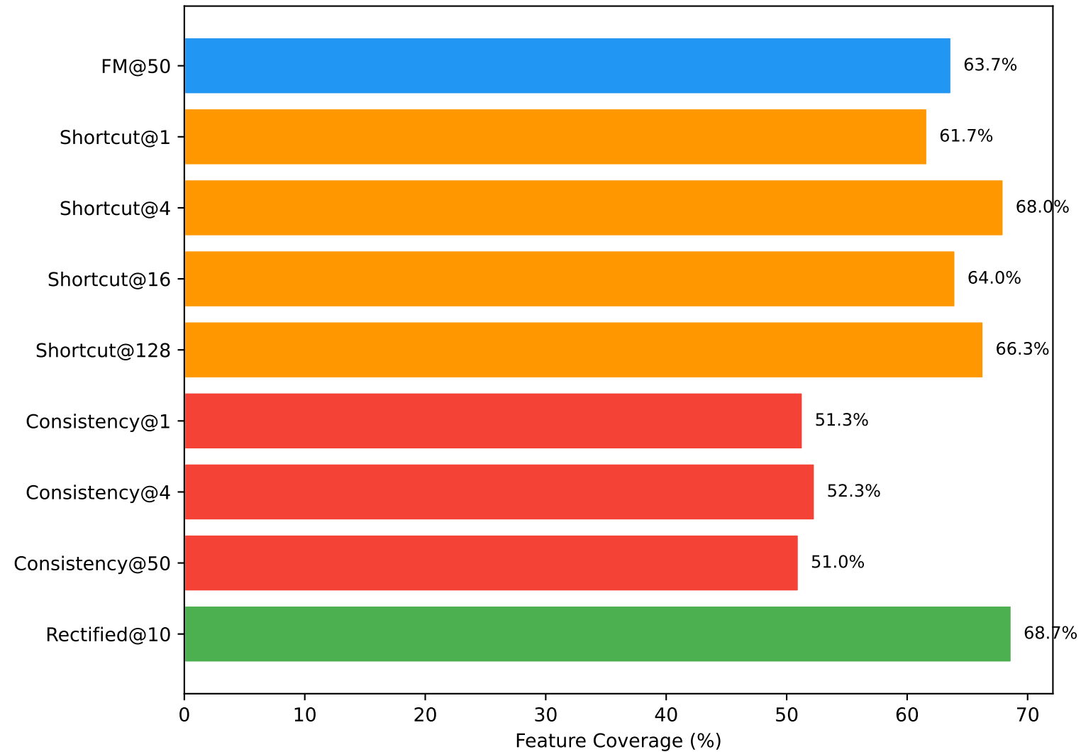
Coverage of Real Feature Space
