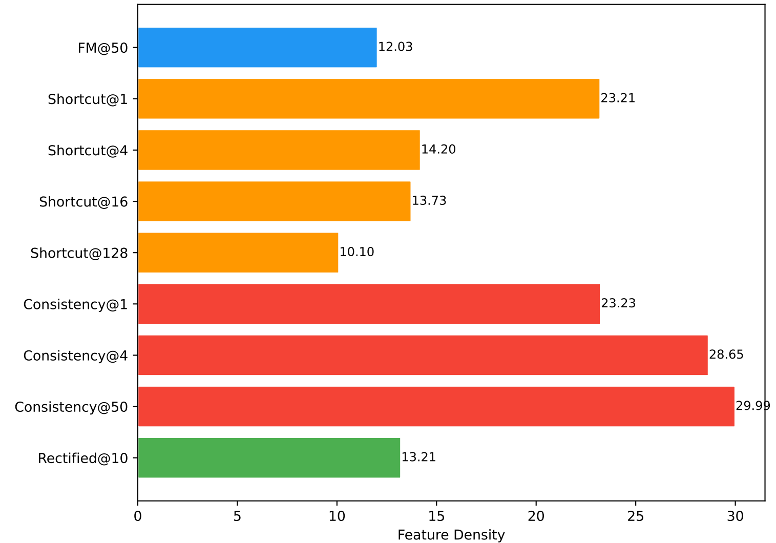
Density in Real Feature Space
