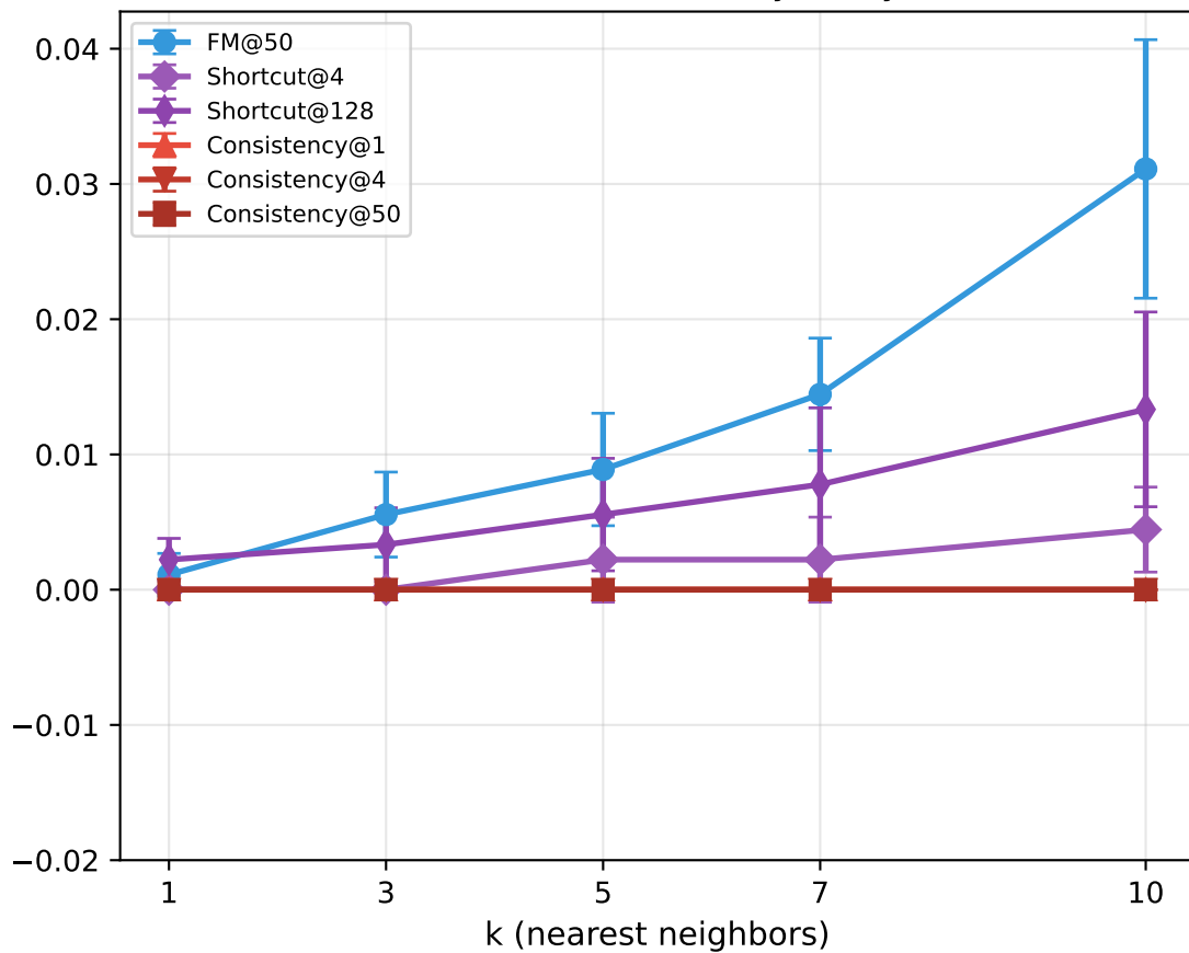
Recall vs k — Sensitivity Analysis
