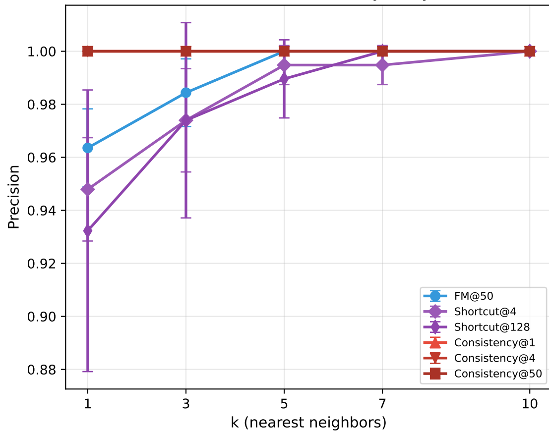
Precision vs k — Sensitivity Analysis
