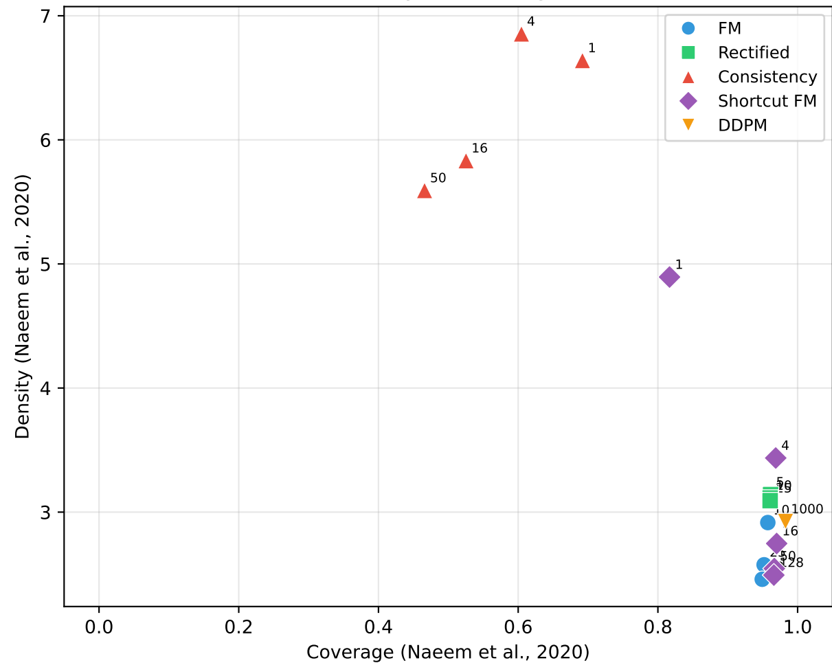
Density vs Coverage
