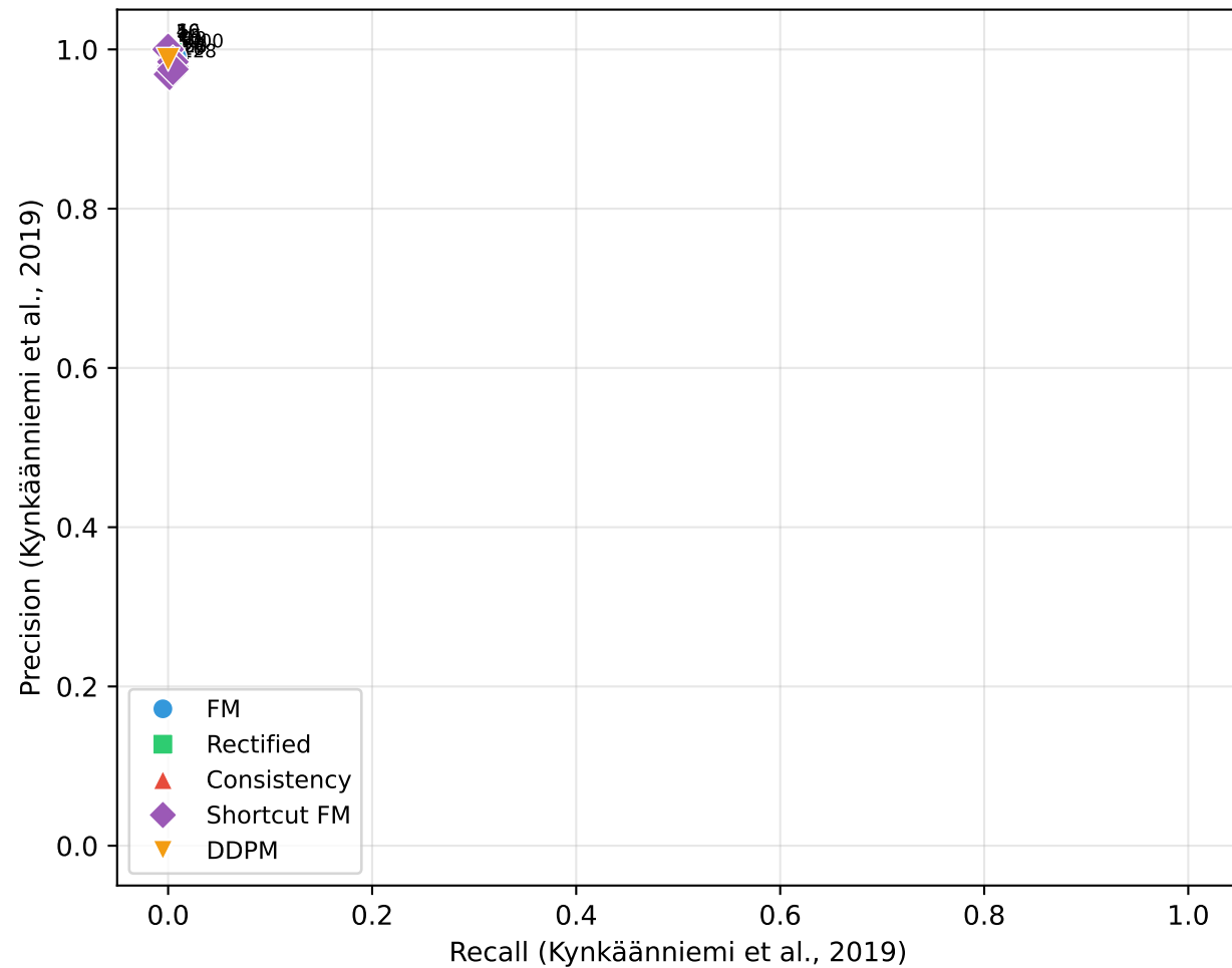
Precision vs Recall
