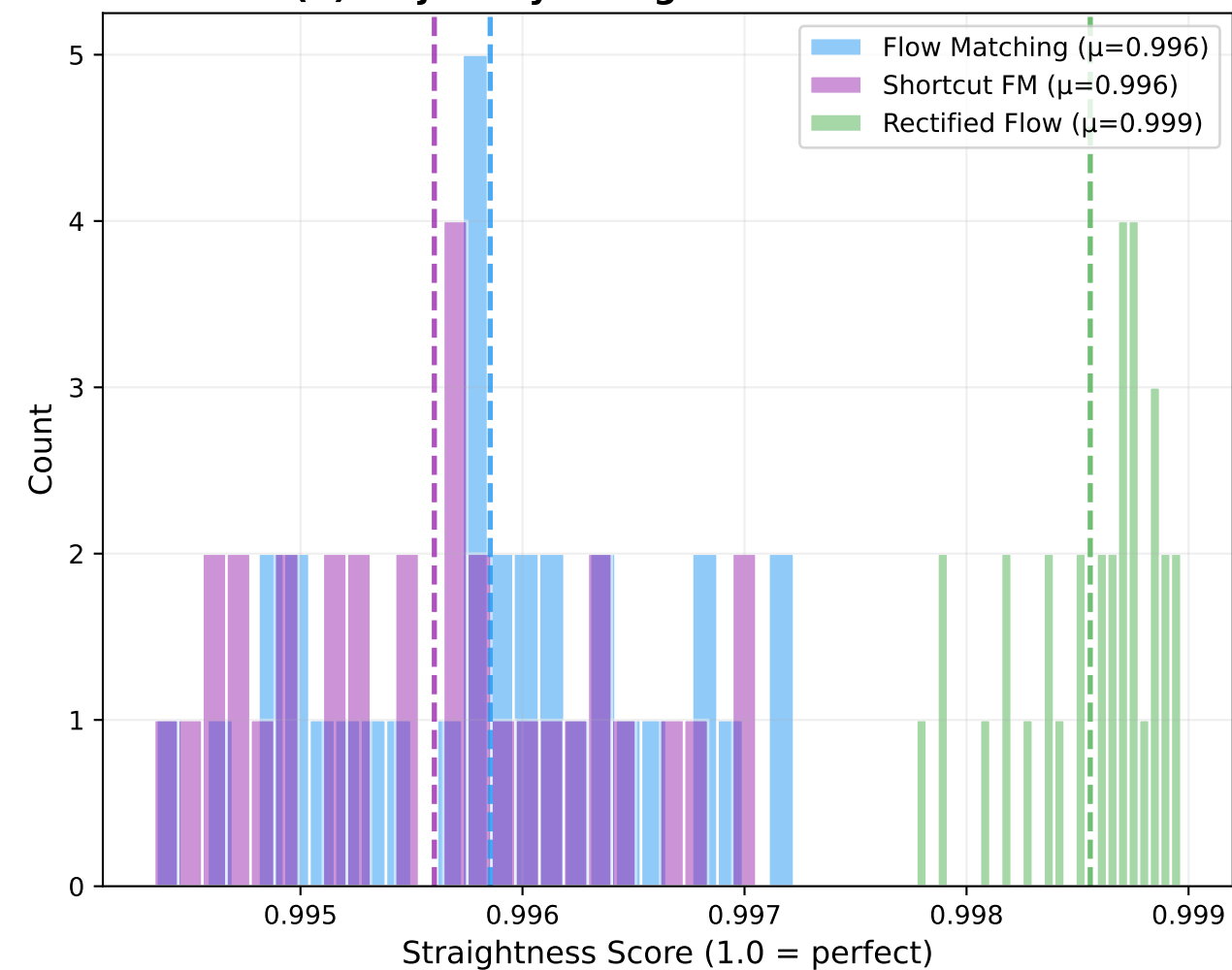
(b) Trajectory Straightness Distribution
