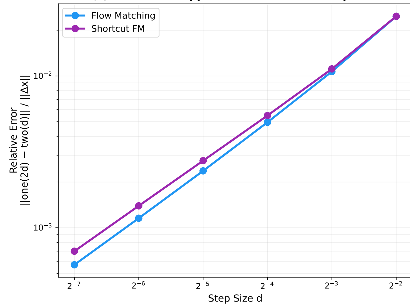
(c) First-Order Approximation Error vs Step Size
