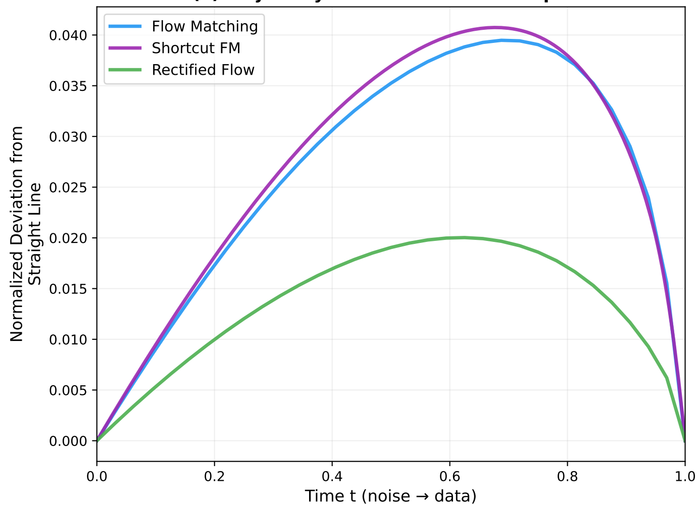
(a) Trajectory Curvature in Latent Space
